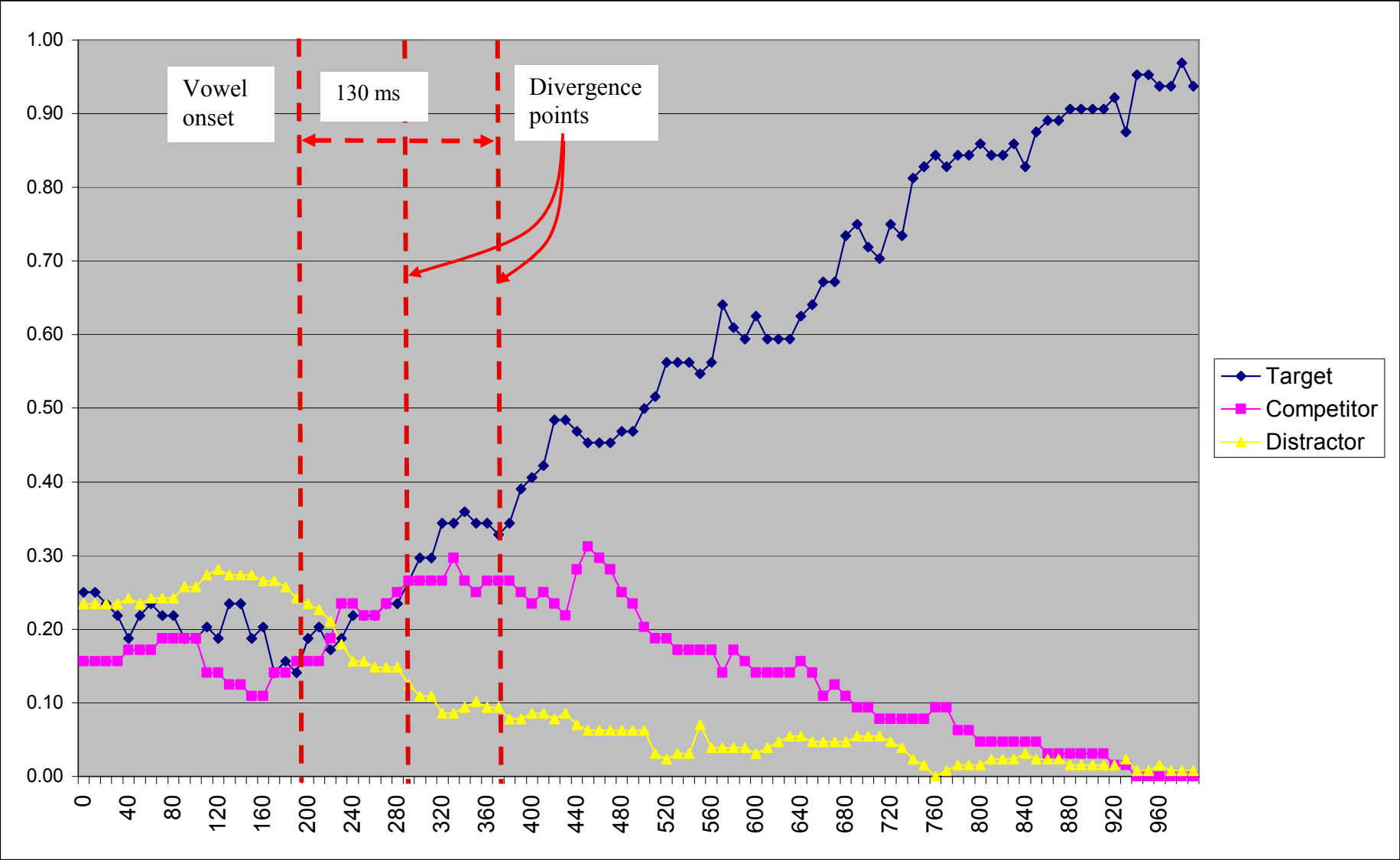
7. Average fixation curves for JCCV words with unrounded vowels
