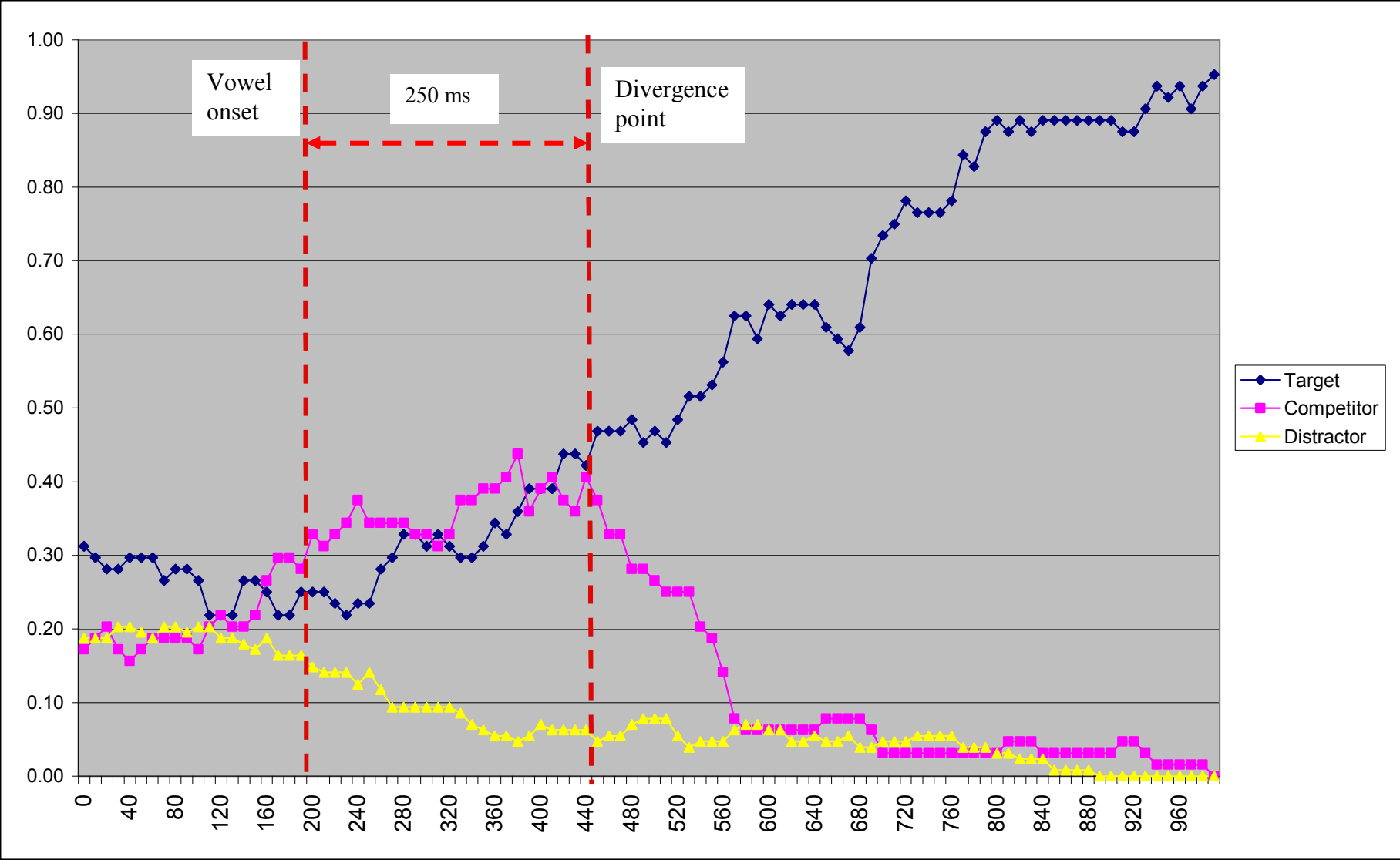
6. Average fixation curves for JCCV words with unrounded vowels
